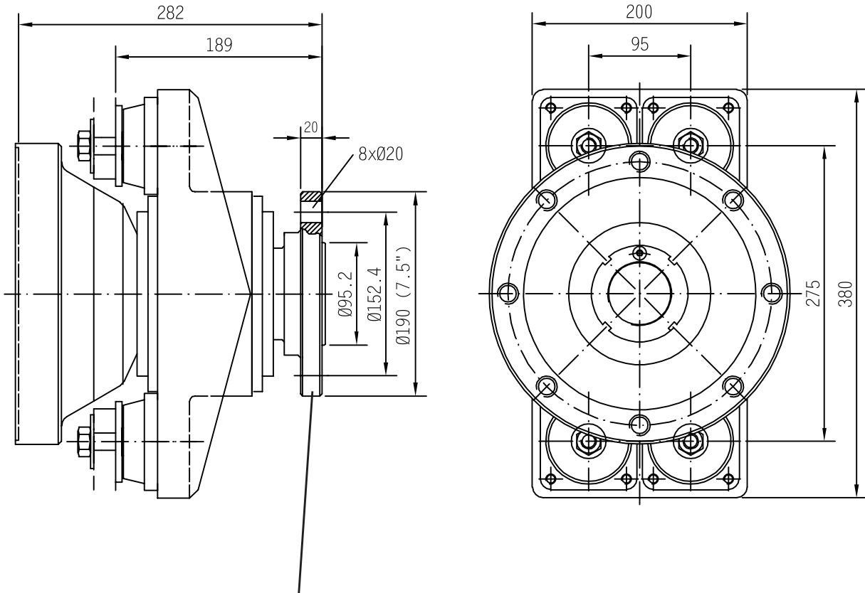
Suits Twin Disc std prop flange PX9153 Passar Twin Disc std prop flange PX9153
